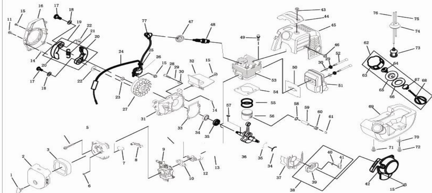
FIG. 1: 1E34F GASLINE ENGINE
