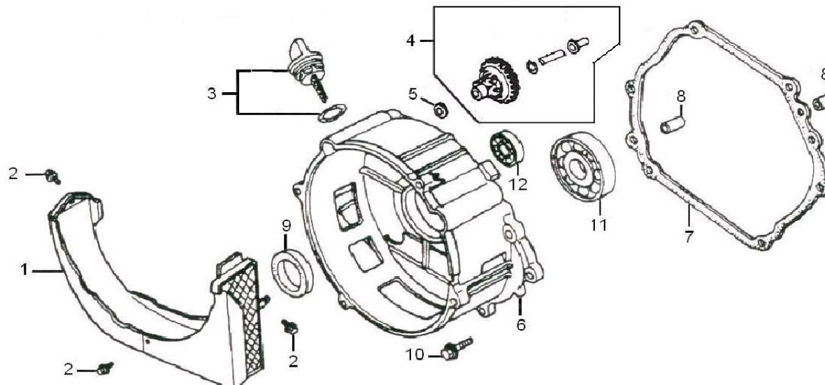
( Crankcase cover )
