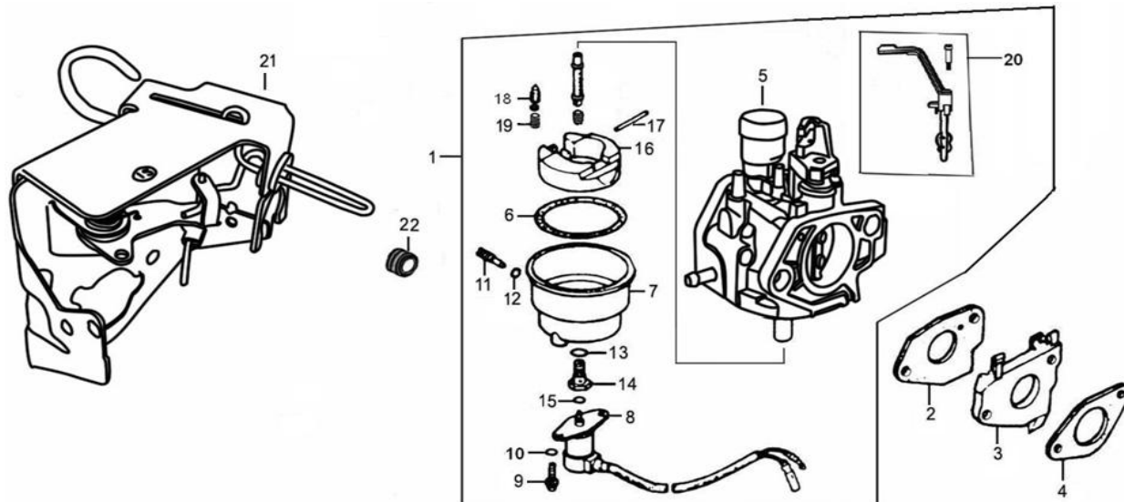
( Carburetor )
