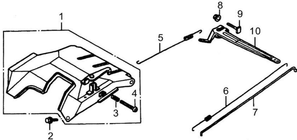
( Control )
