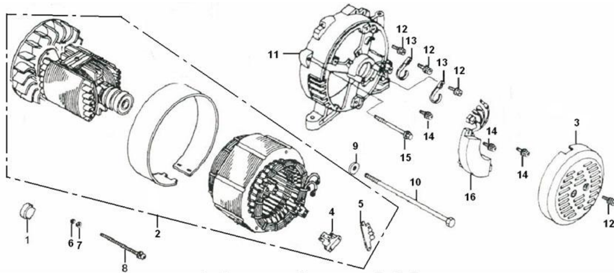
( Stator/Totor/Housing )
