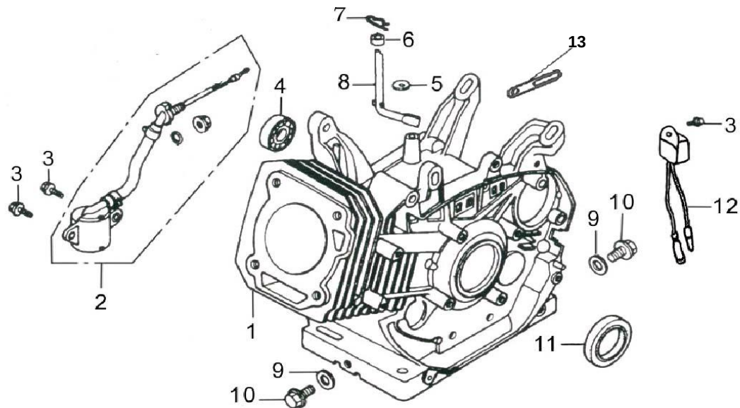
( Crankcase )
