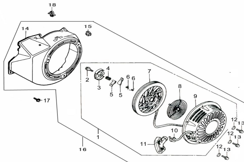
( Starter )
