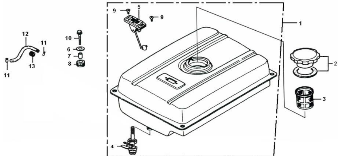
( Fuel tank )
